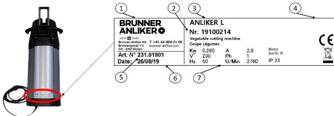
Fig. 1: Nameplate
